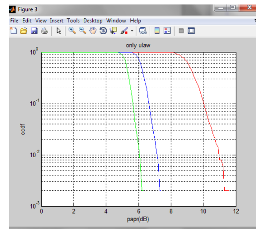
Figure3:Companding technique
