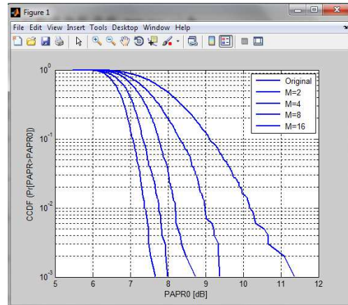
Figure3: Selective Mapping; for m, m=16 we got reduction in PAPR
